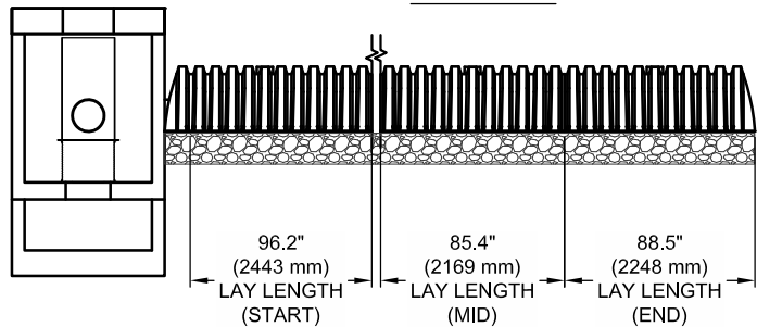
ELEVATION VIEW
